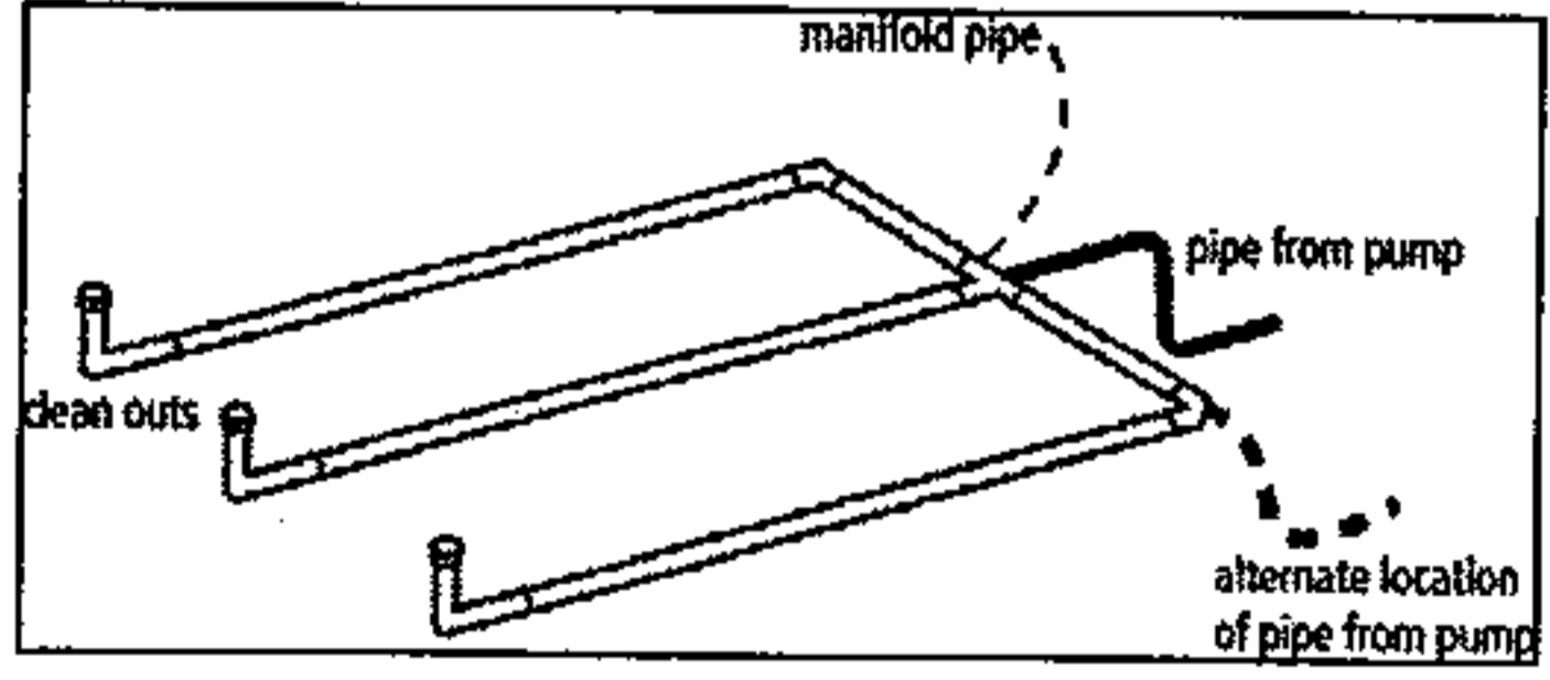
END Connection
